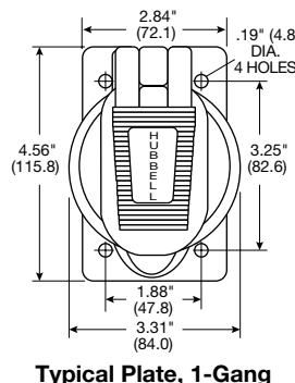
Typical Plate, 1-Gang
