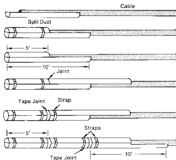
The fast and easy method of installing duct around existing cable for repair and temporary installations.
