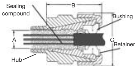
With bushing
